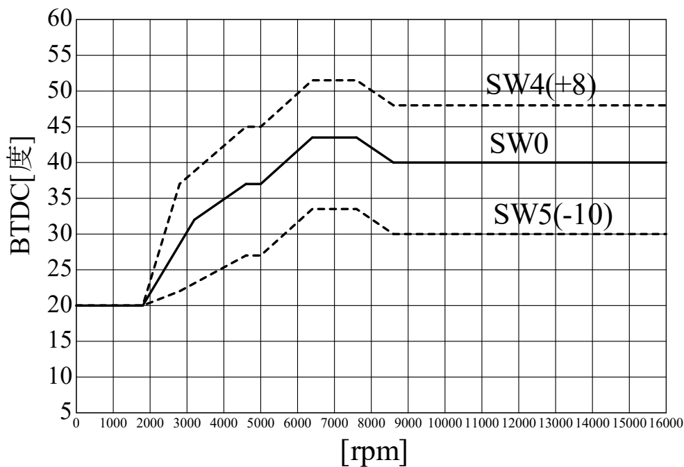
SP2FPKit(S.GSX250S) ignition curve
