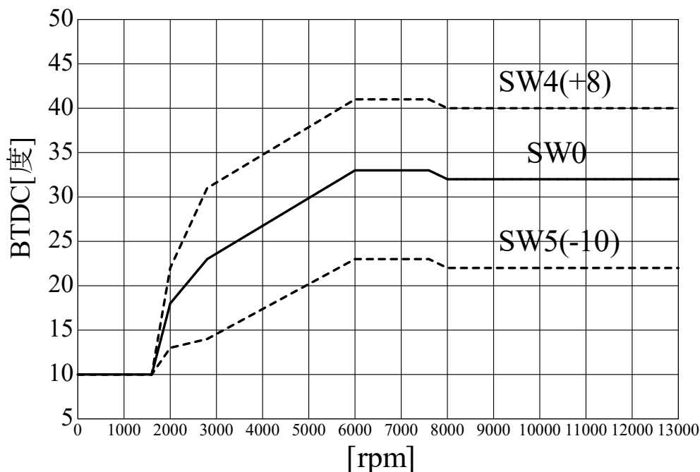
SP2FPKit(S.GSX400S) ignition curve
