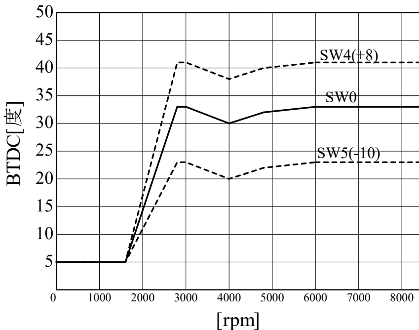
SP2FPKit (K.W1/3) ignition curve AS UOTANI
