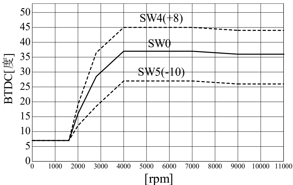
SP2FPKit(Y.XJ750E) ignition curve
