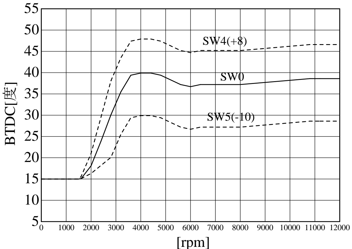
SP2FPKit (H.V45MAGNA) ignition curve AS UOTANI
