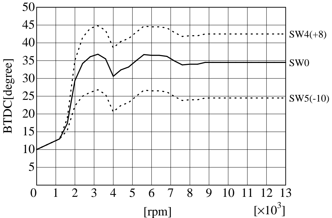
SP2FPKit (S.GSF1200) ignition curve AS UOTANI
