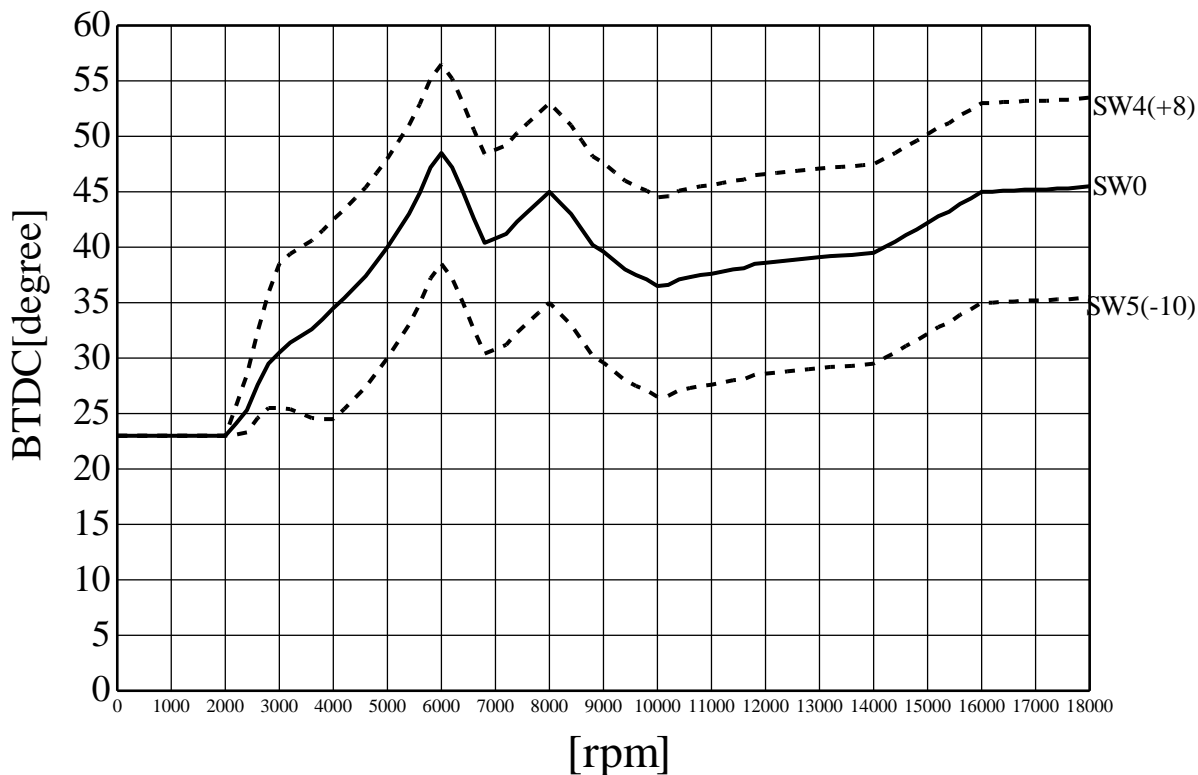
SP2FPKit(BALIUS-1) ignition curve AS UOTANI
