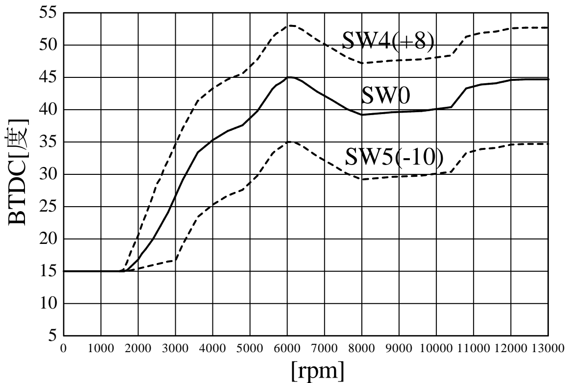
SP2FPKit(H.VFR750R) ignition curve
