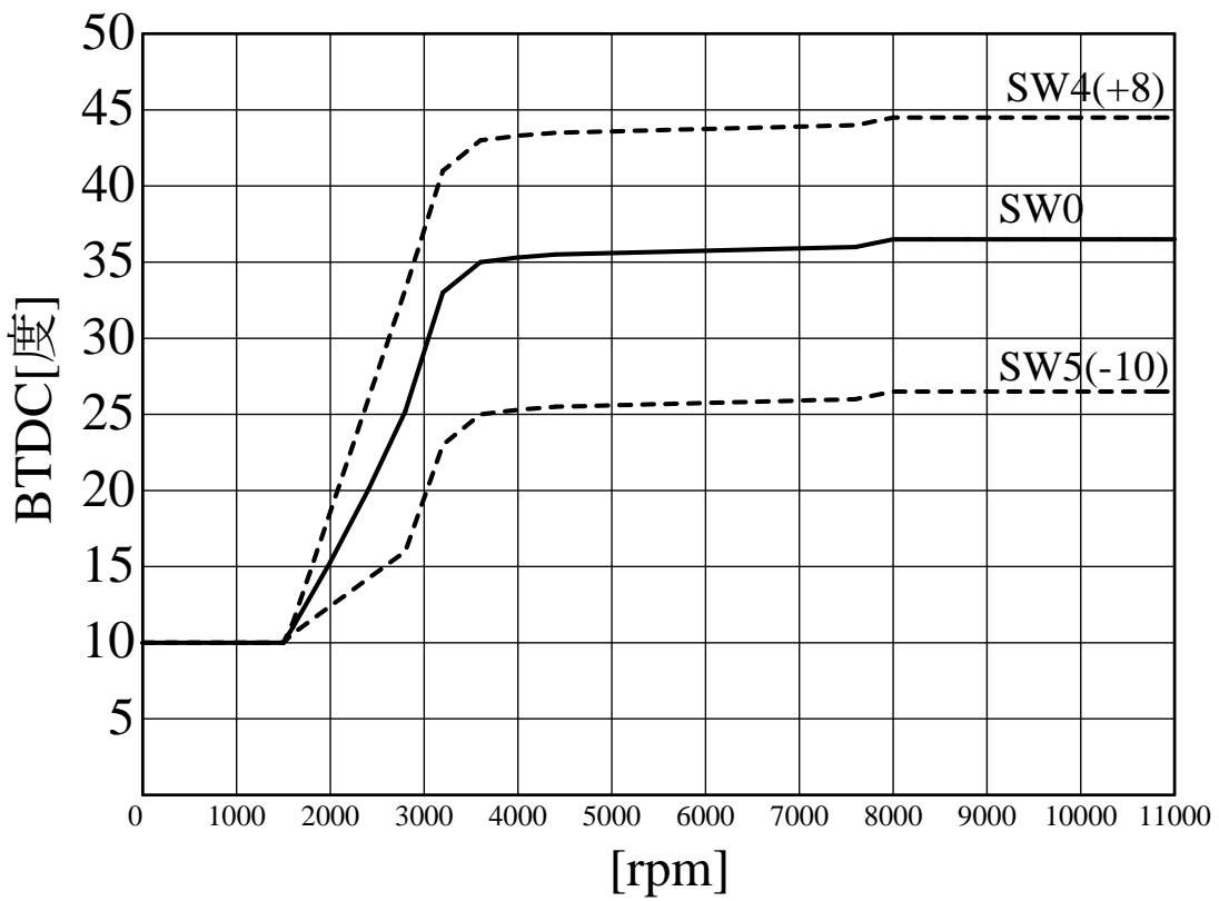
SP2FPKit (H.CBX750F) ignition curve AS UOTANI
