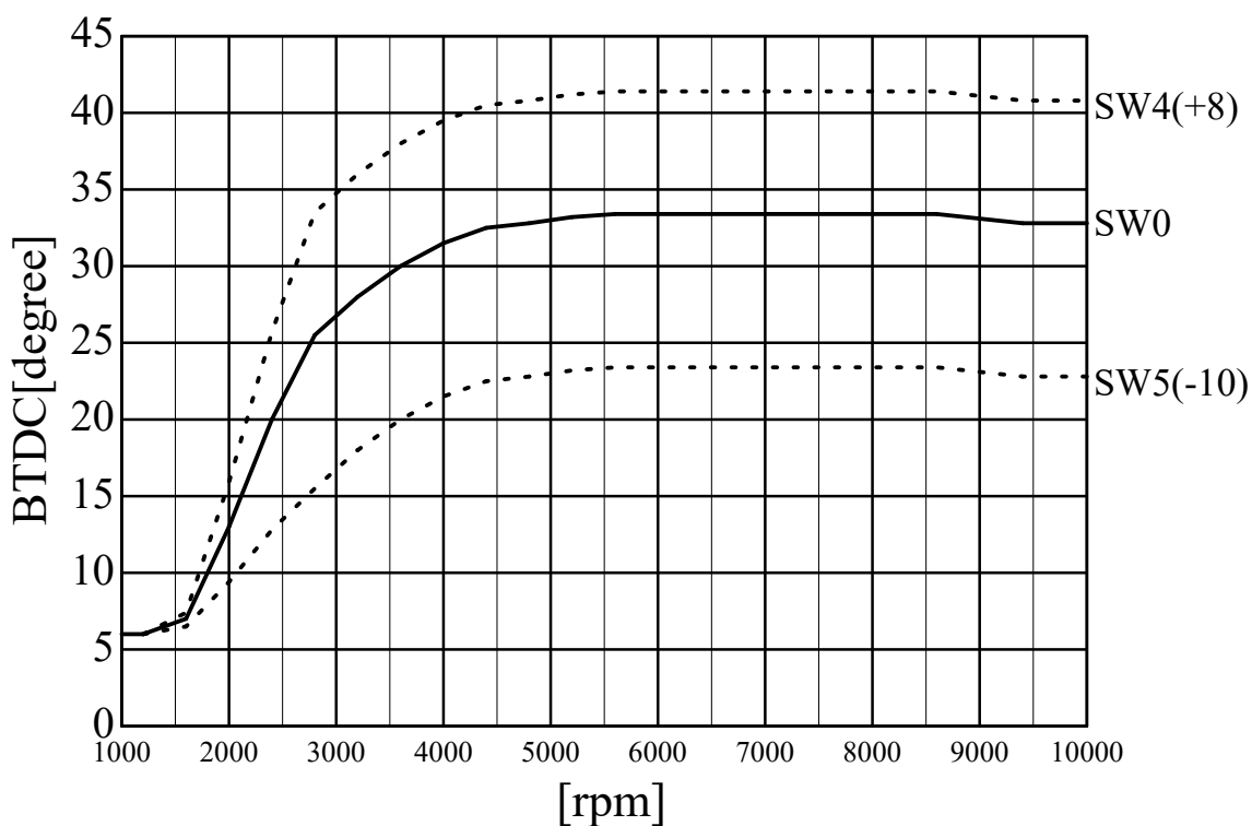
SP2FPKit (D.M900/SS) ignition curve AS UOTANI
