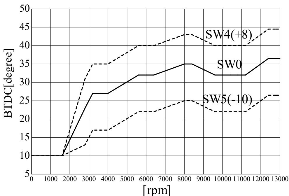
SP2FPKit(S.GSX400 IMPLUSE-1) ignition curve
