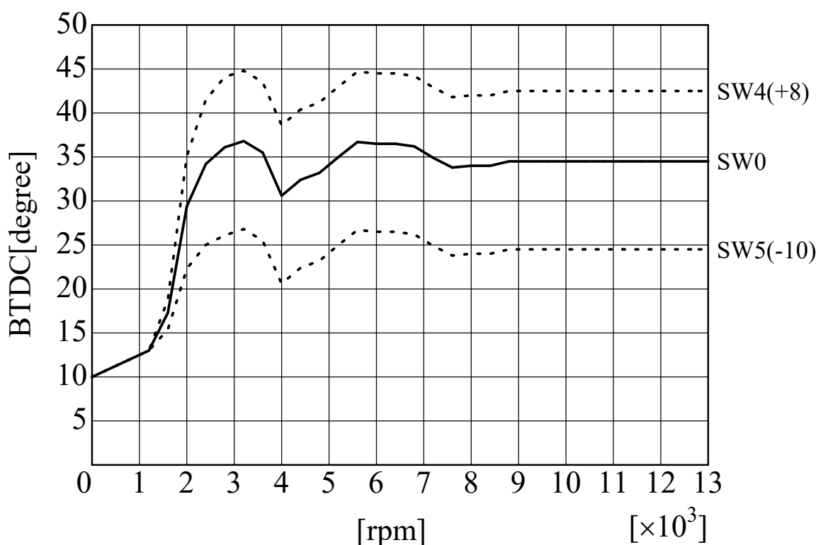
SP2FPKit (S.GSF1200) ignition curve AS UOTANI
