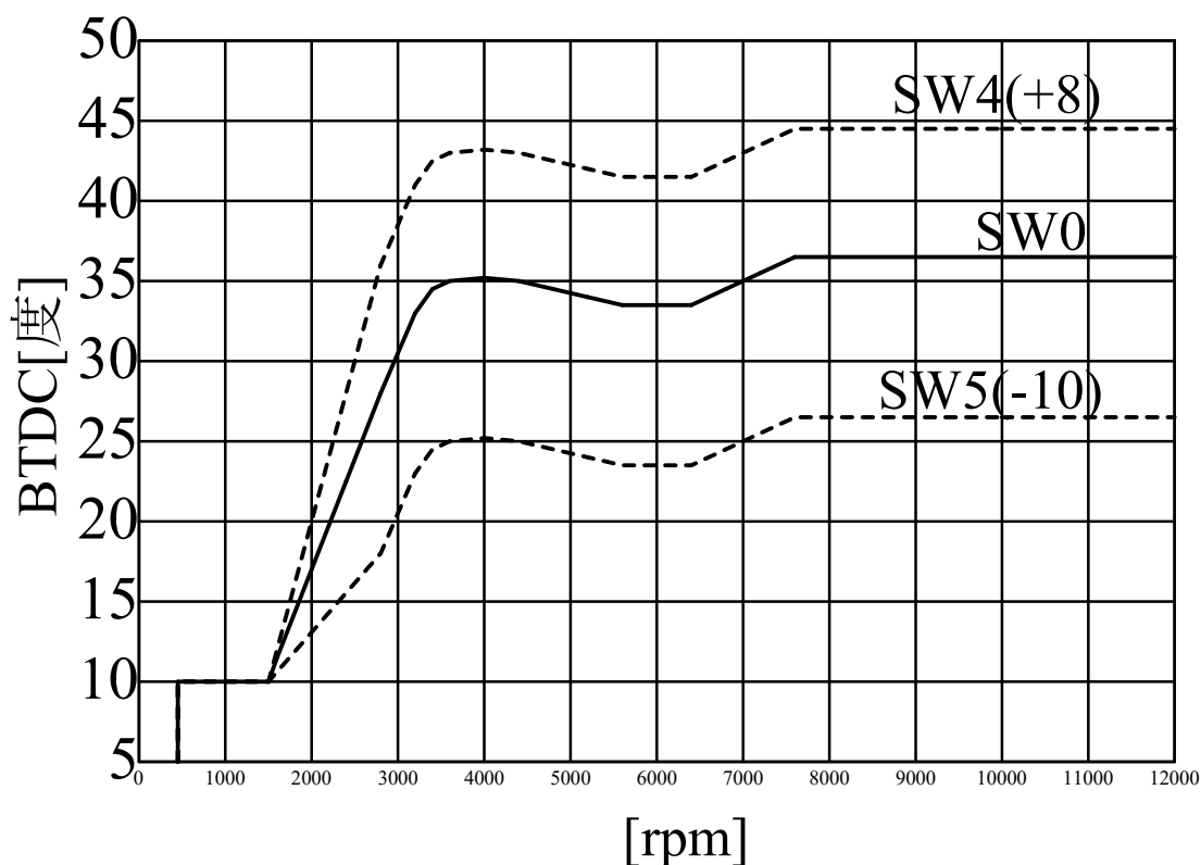
SP2FPKit(K.Z400FX) ignition curve
