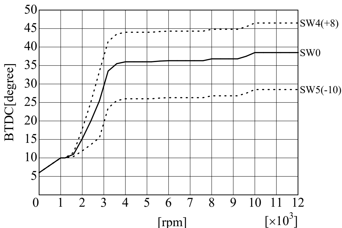
SP2FPKit (K.GPZ900R-2) ignition curve AS UOTANI
