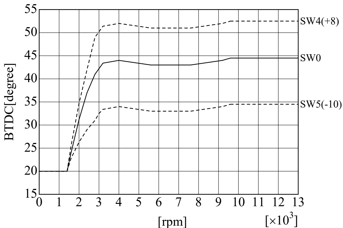
SP2FPKit (H.CBR400F) ignition curve AS UOTANI
