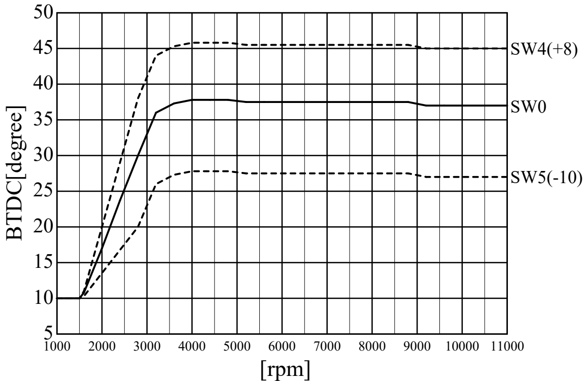
SP2FPKit (H.VF750F) ignition curve AS UOTANI
